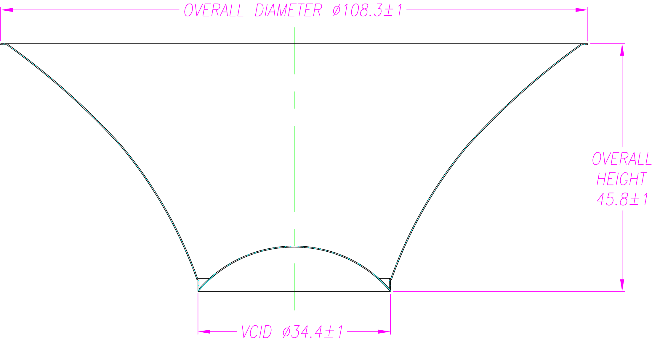
WHIZZER CONE-WC110A
