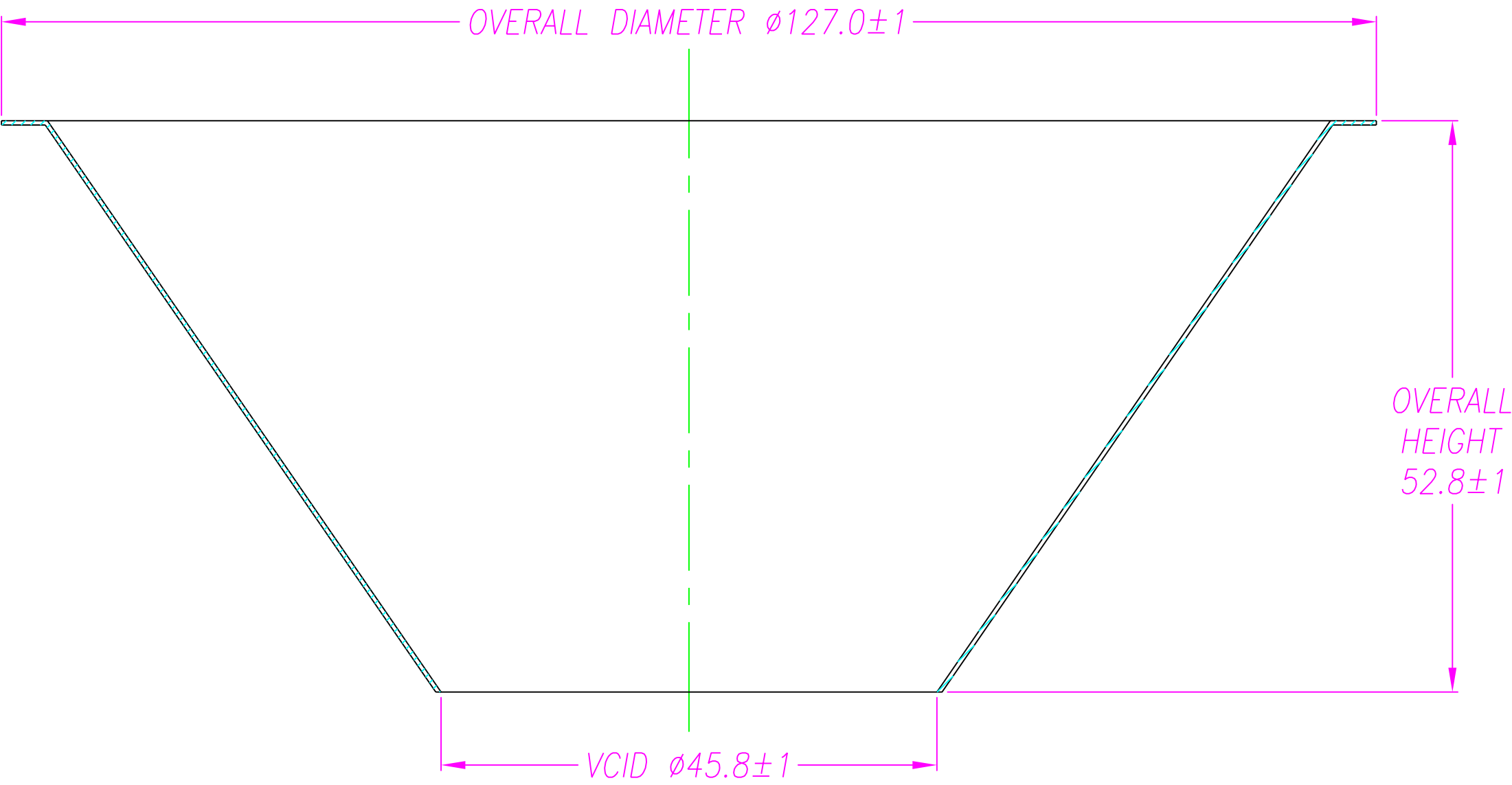
WHIZZER CONE-WC127A2
